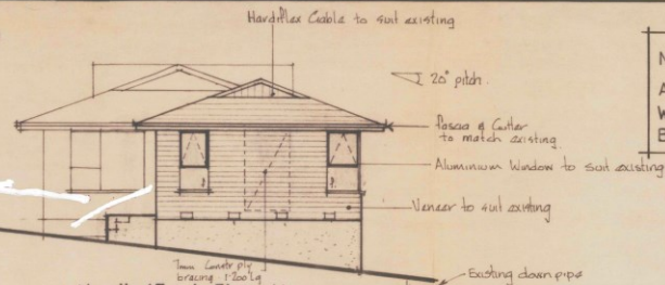
North/East Elevation
