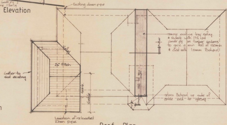
Roof Plan
