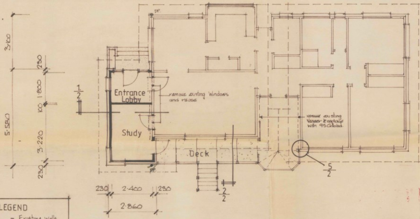
Floor Plan
