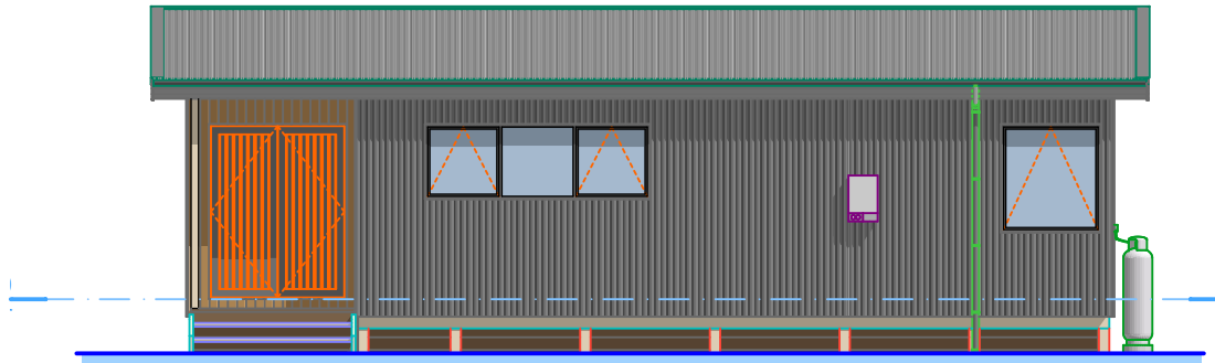
A Elevation 1:100
